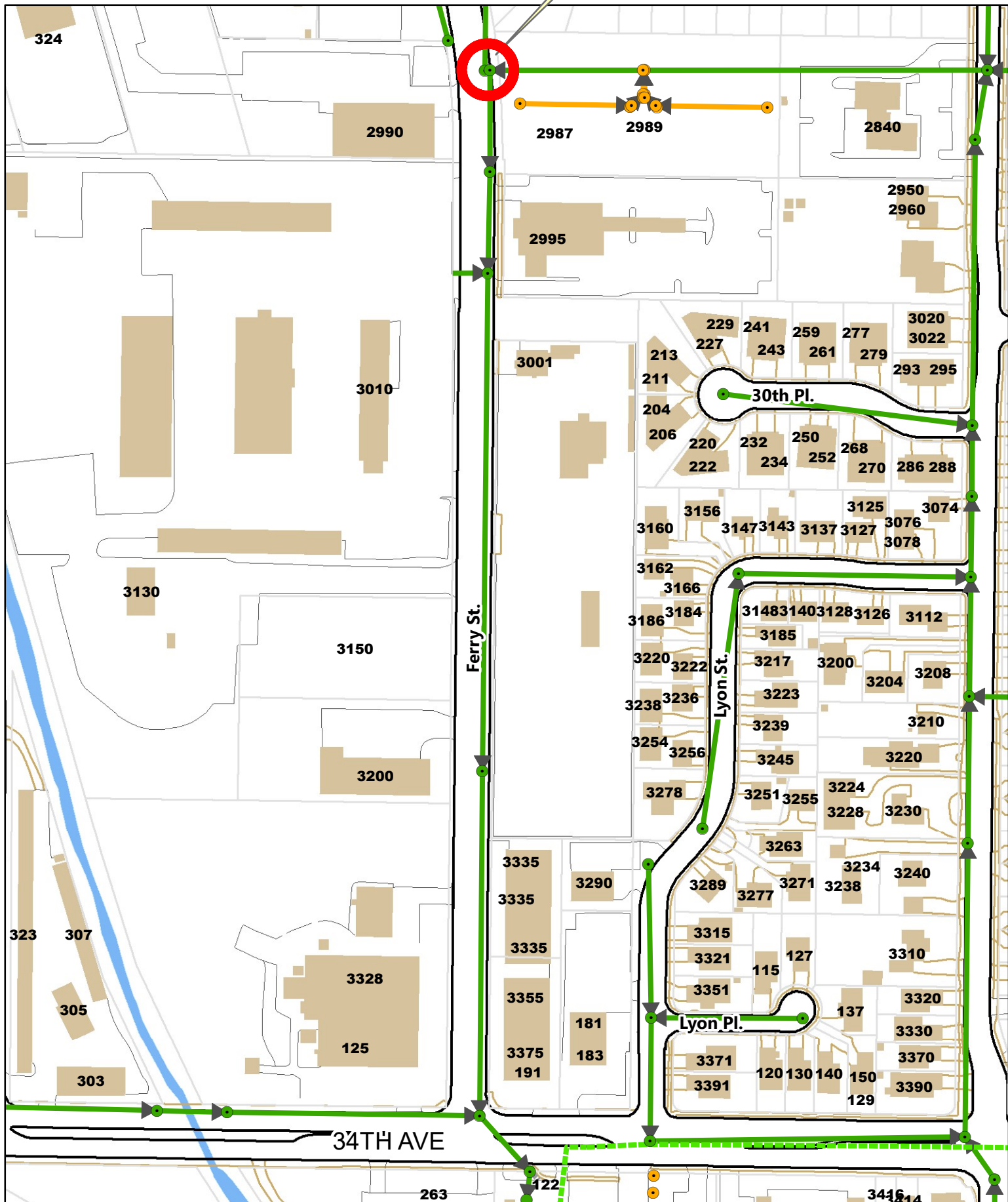
ADDENDUM 1 ATTACHMENT 2: BYPASS MANHOLE LOCATION MAP
